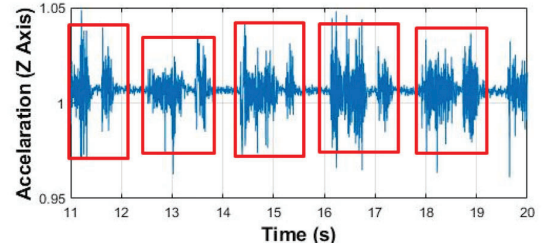
(c) Speech region detection from accelerometer data for loudspeaker setting
