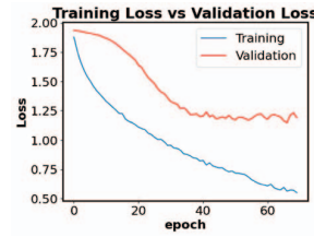
(c) Emotion recognition ear speaker training loss Vs. validation loss for TESS dataset.
