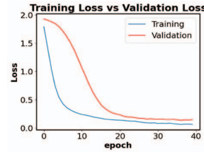
(a) Emotion recognition loudspeaker training loss Vs. validation loss for TESS dataset.
