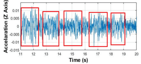
(b) Speech Region detection from accelerometer data for earpiece setting after applying 8Hz high-pass filter.
