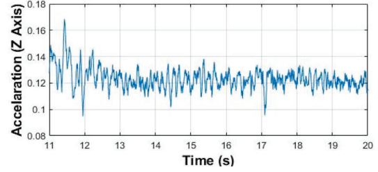
(a) Raw accelerometer data for earpiece setting (no trace for speech region)
